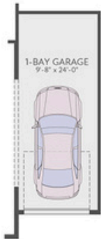
OPT. 1-BAY GARAGE EXTENSION
