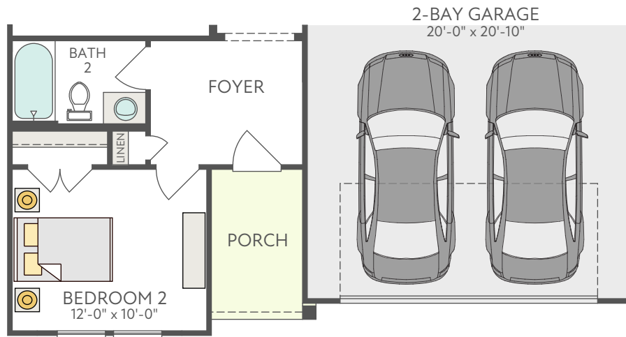
FIRST FLOOR EXTERIOR STYLE B
