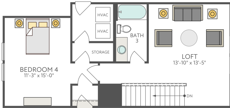
OPT. SECOND FLOOR EXTERIOR STYLE A
