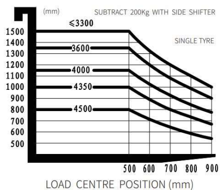
RATED CAPACITIES AND LOAD CENTERS GRAPH
