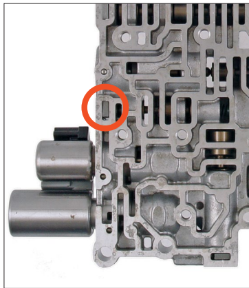
Solenoid Body
