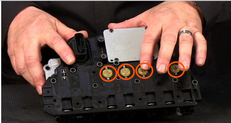
GEN1 units are identified by the existence of (4) pressure switches in the TEHCM.
