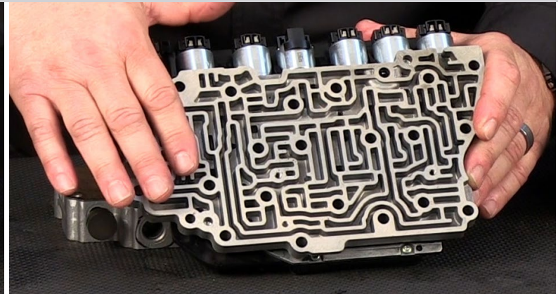
When you split the valve body, GEN1 units have no pulse dampeners.
