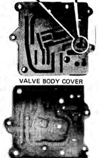
SMALL SEPARATOR PLATE
