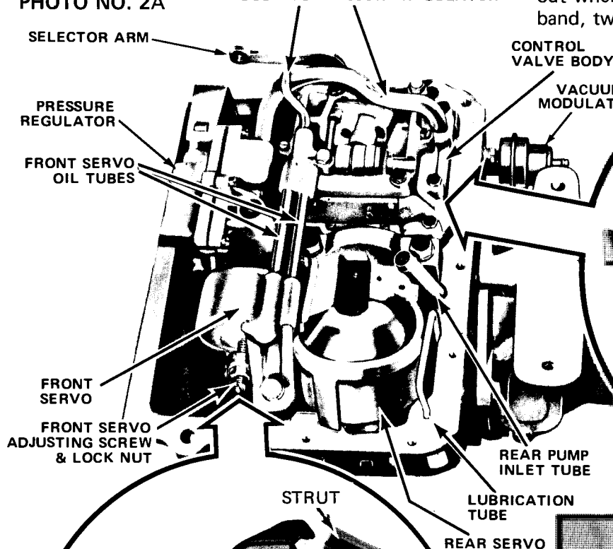
PHOTO NO. 2A REMOVE THESE TWO TUBES CONNECTING VALVE BODY TO PRESSURE REGULATOR
