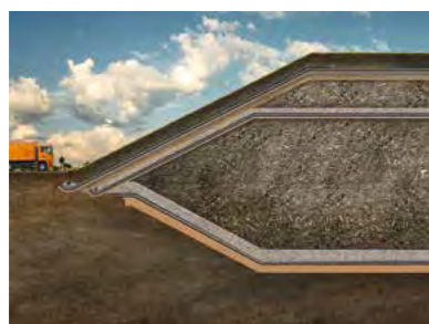
Landfill Construction
