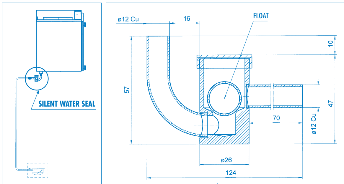
Vallox water seal "SILENT"
