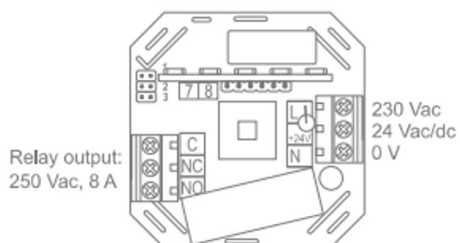
Koppling
