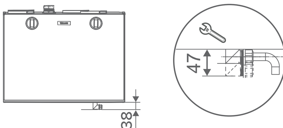
Figure 3. Space required by the alternative Vallox Silent Klick water seal installation method (elbow)
