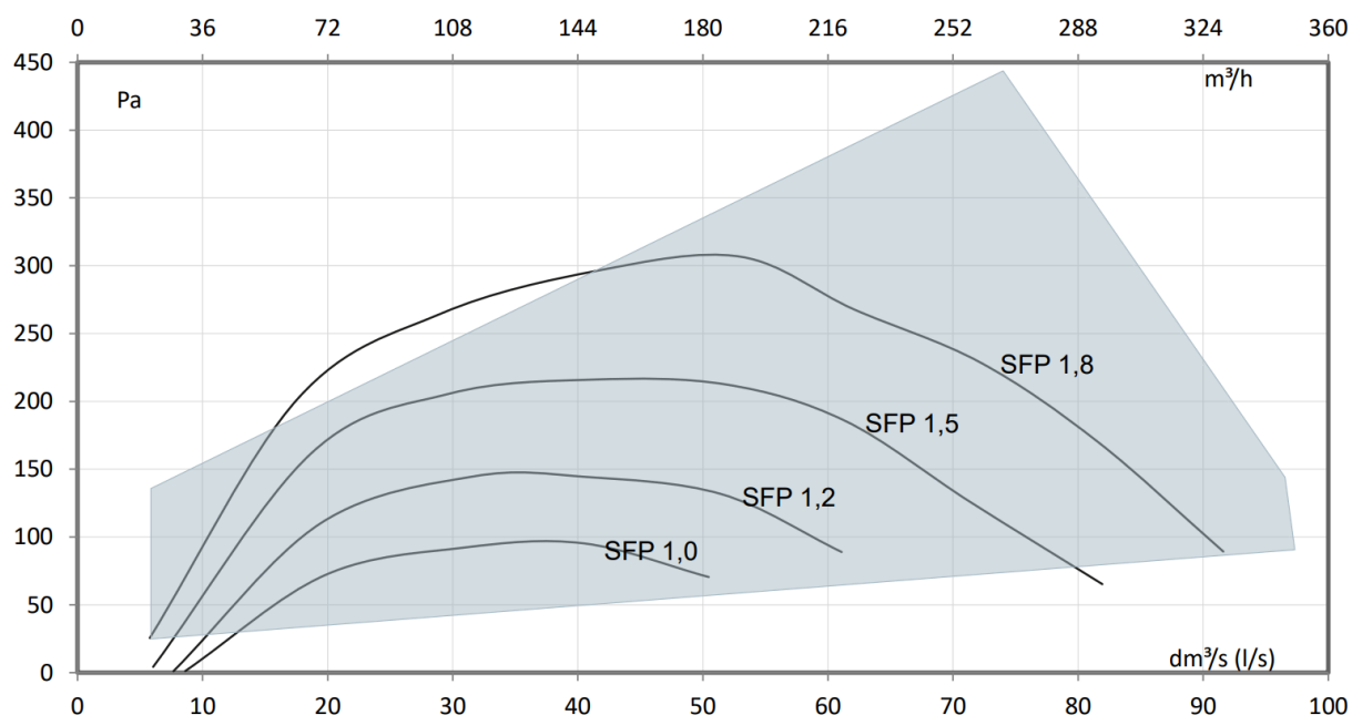
Figure 6. Fan supply and extract air volumes, enthalpy heat recovery cell
