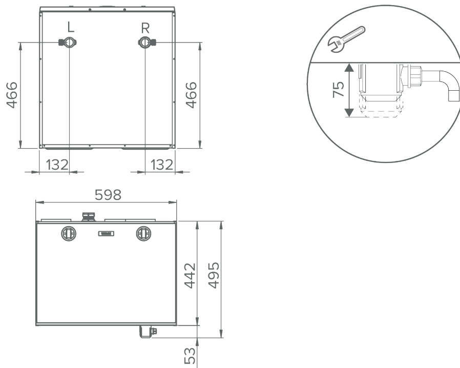
Figure 3. Space required by the alternative Vallox Silent Klick water seal installation method (elbow)
