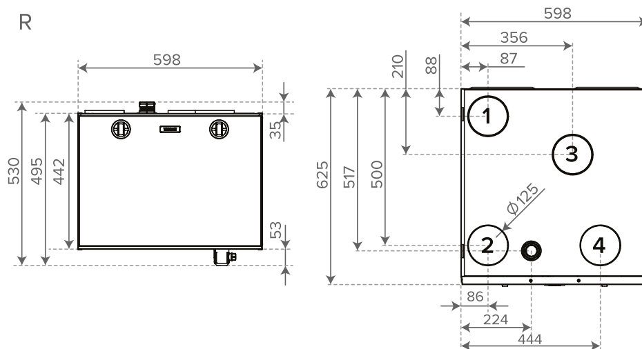
Figure 10. Dimensions and duct outlets MyVallox 99 CFi L
