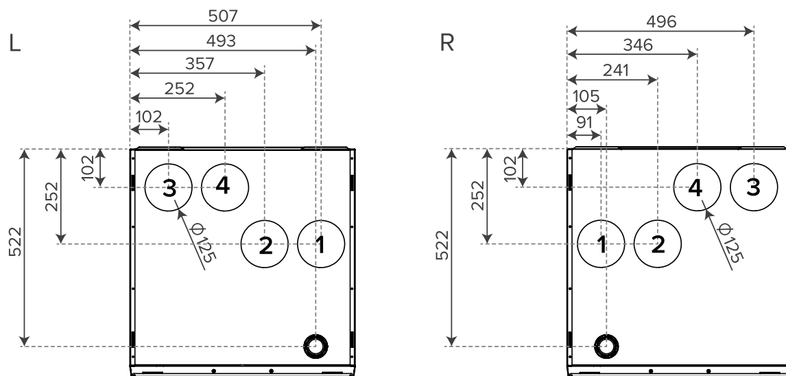
Figure 14. Dimensions and duct outlets 125G
