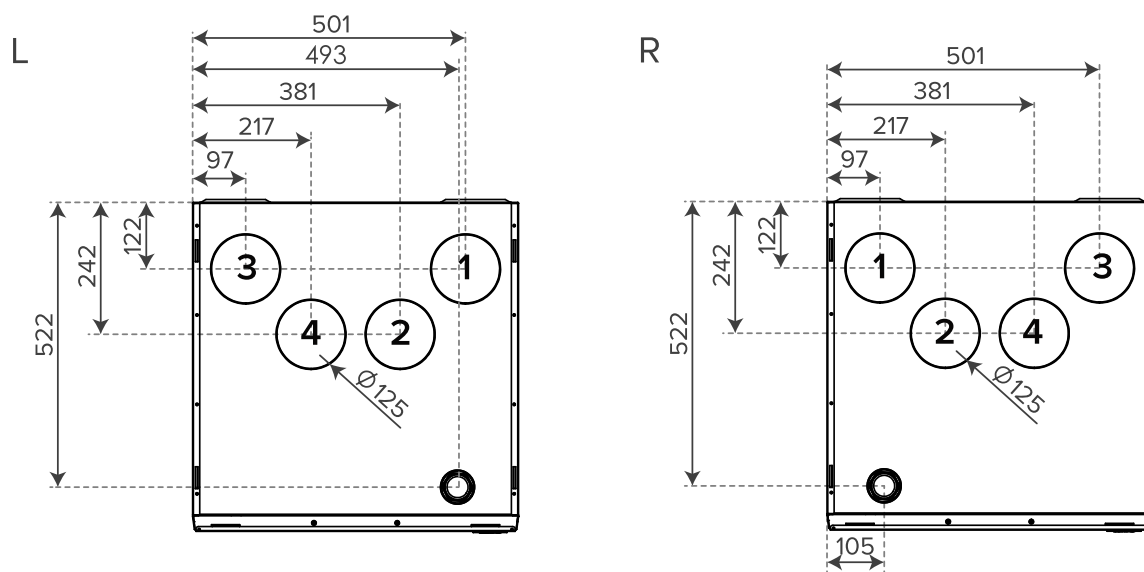
Figure 12. Dimensions and duct outlets 125E
