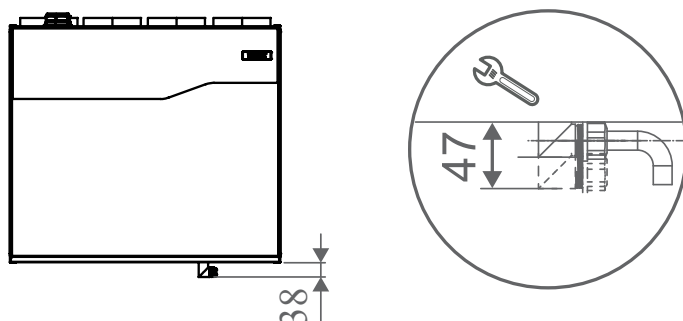
Figure 8. Dimensions and duct outlets 125A
