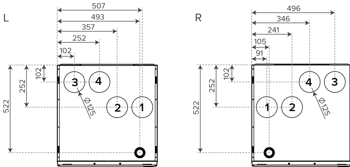
Figure 13. Dimensions and duct outlets 125G
