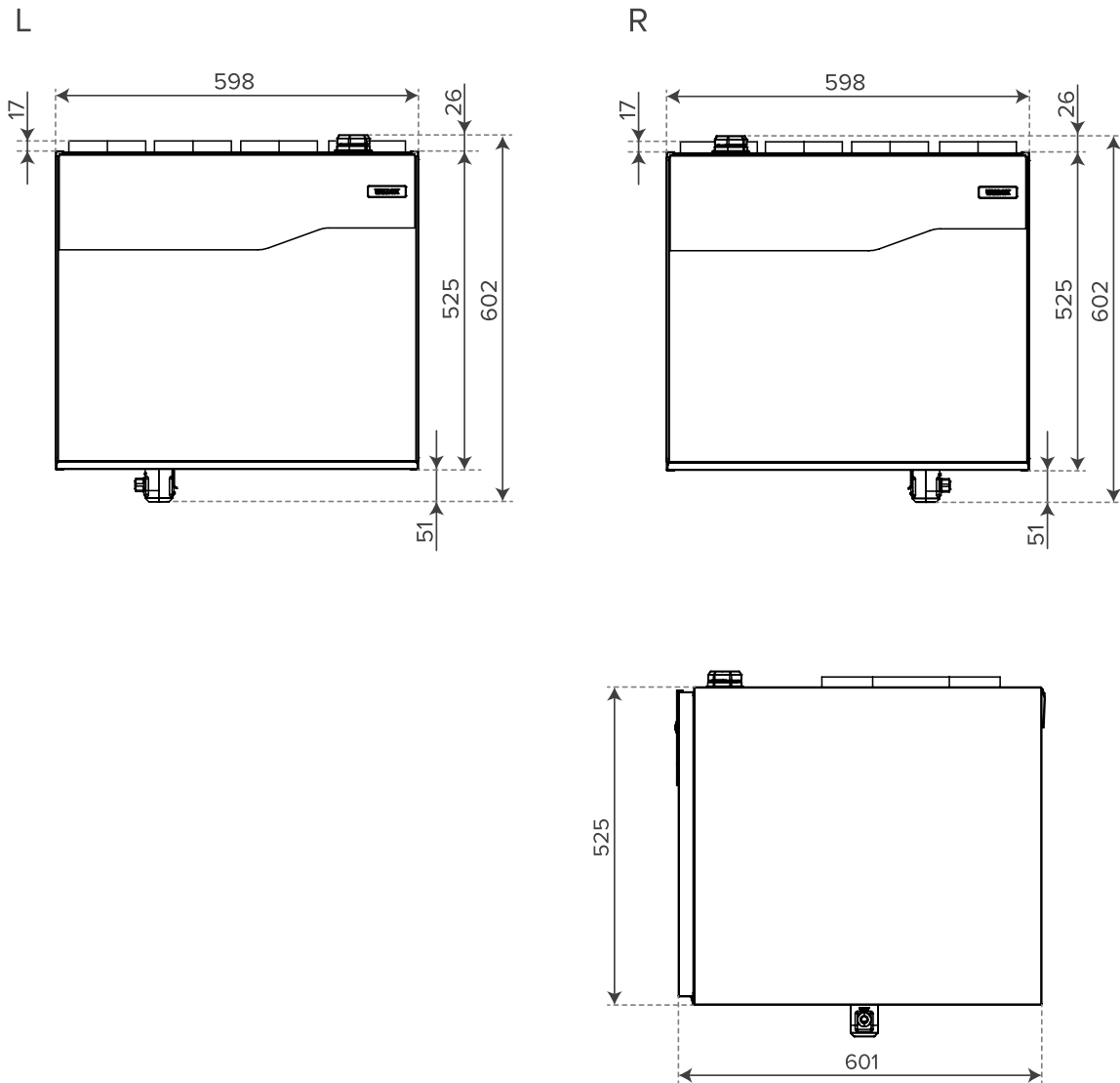
Figure 6. Dimensions MyVallox 125 CFI
