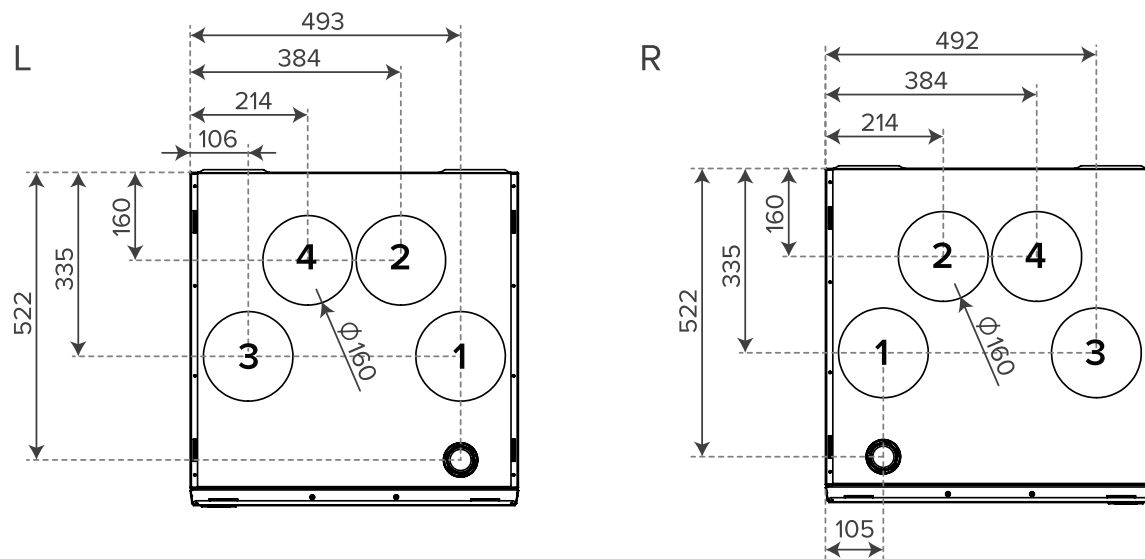
Figure 14. Dimensions and duct outlets 125H
