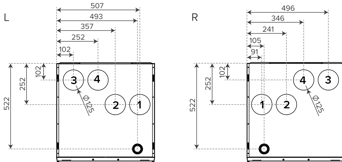
Figure 13. Dimensions and duct outlets 125G
