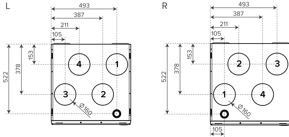
Figure 10. Dimensions and duct outlets 125D
