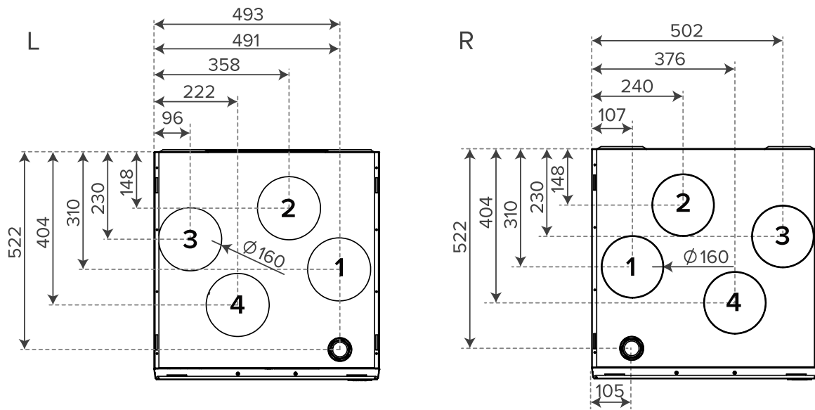
Figure 12. Dimensions and duct outlets 125F
