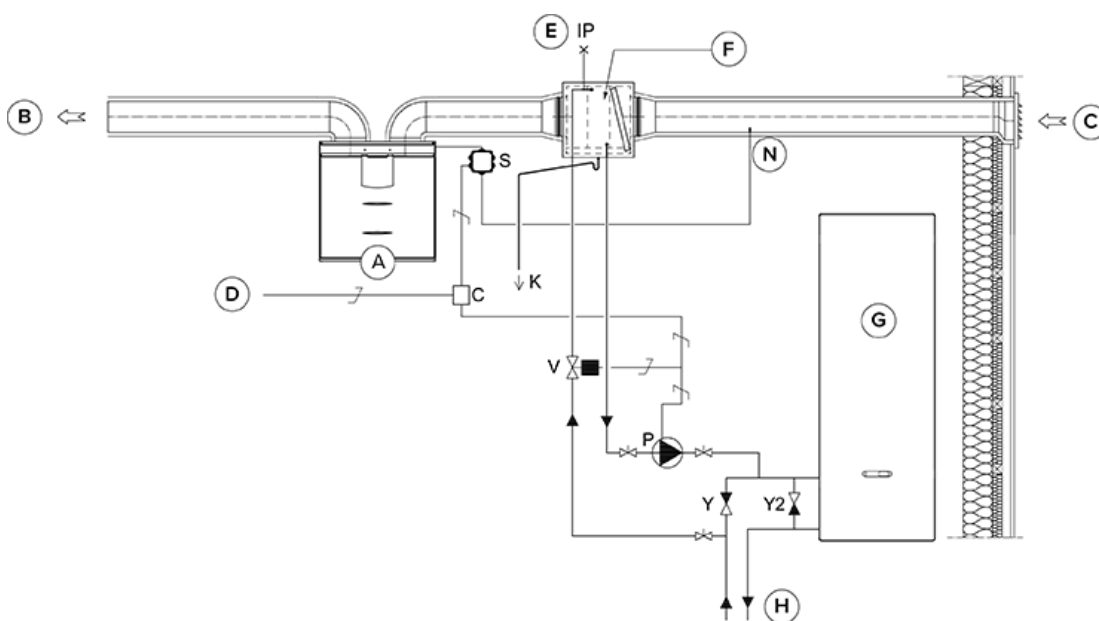
Figure 6. Duct radiator operation chart in the outdoor air duct
