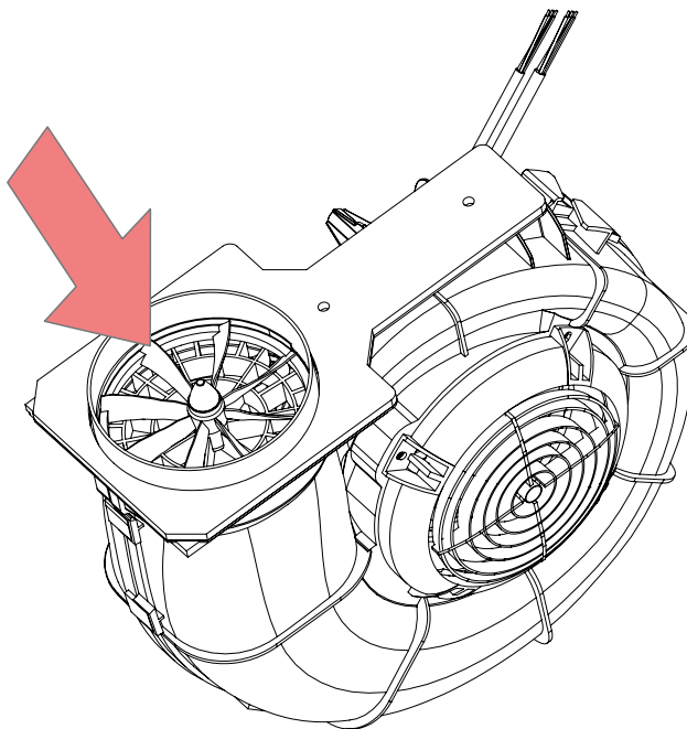
Figure 3. Cleaning the anemometer
