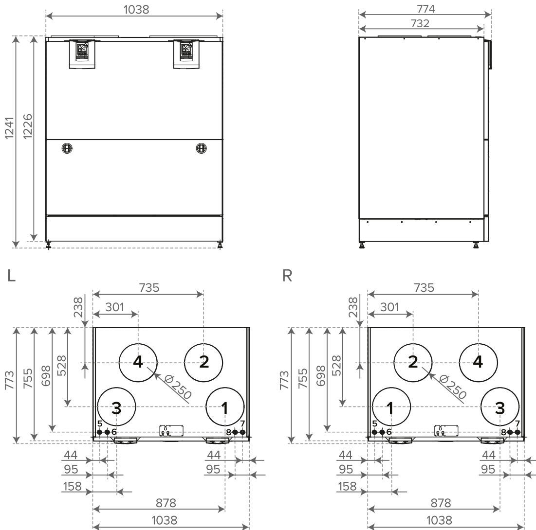
Figure 6. Dimensions
