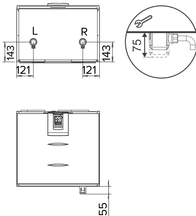
Figure 2. The space required by the alternative Vallox Silent Klick siphon installation method (elbow)
