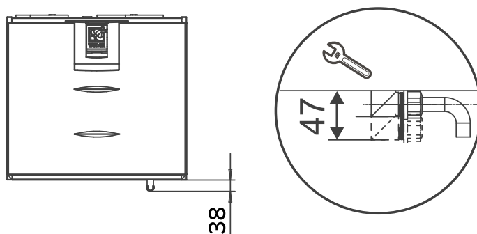
Figure 2. The space required by the alternative Vallox Silent Klick siphon installation method (elbow)
