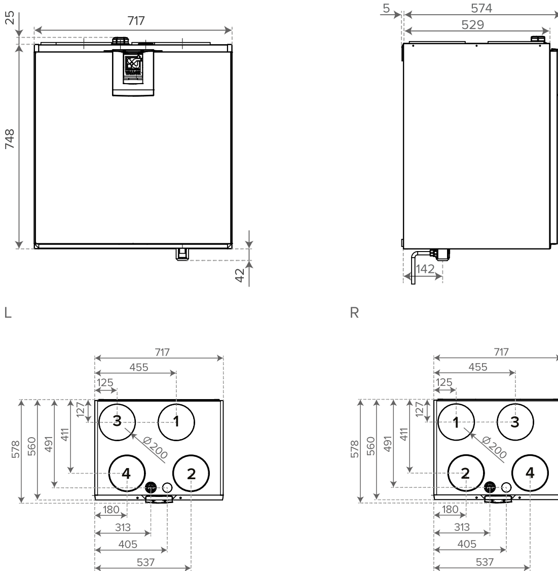
Figure 7. Dimensions and duct outlets
