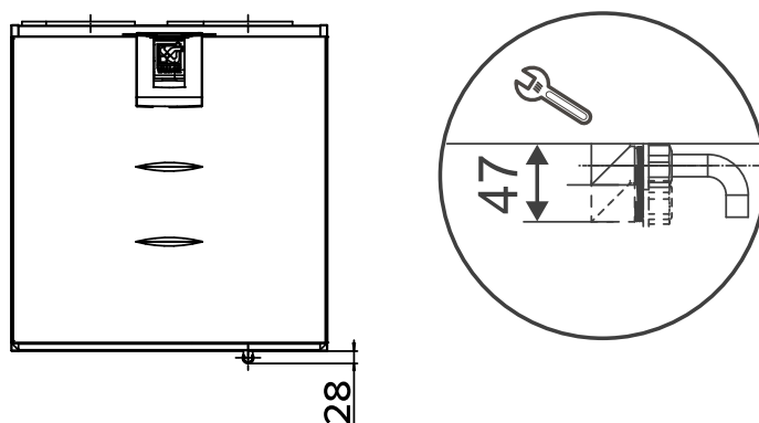
Figure 2. The space required by the alternative Vallox Silent Klick siphon installation method (elbow)
