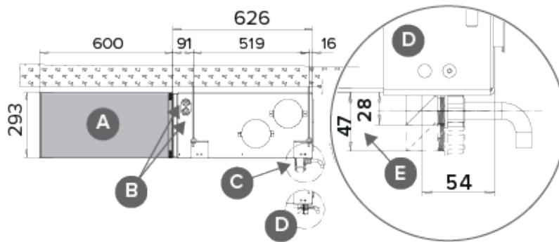
Figure 7. Dimensioning figure and space required for installation of the Vallox Silent Klick siphon
