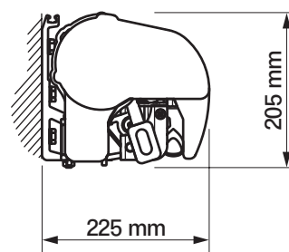
wall installation
