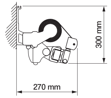
wall installation
