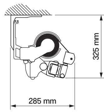
ceiling installation
