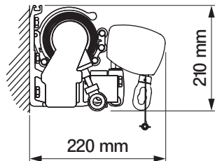
wall installation
