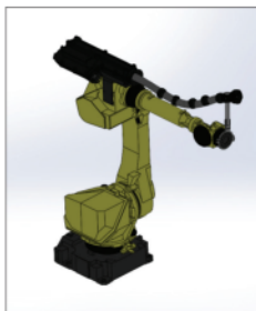
11.48.321.01 Complete robotic dresspack, Axis 3-6, Tecliner retraction system, 350mm stroke, high-flex conduit with ID 64mm
