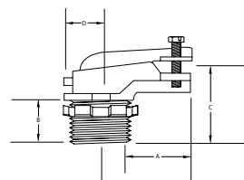
Sizes 3/8" - 3/4" are manufactured as shown above
