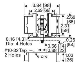
Cabinet Door Type Two Contact Blocks
