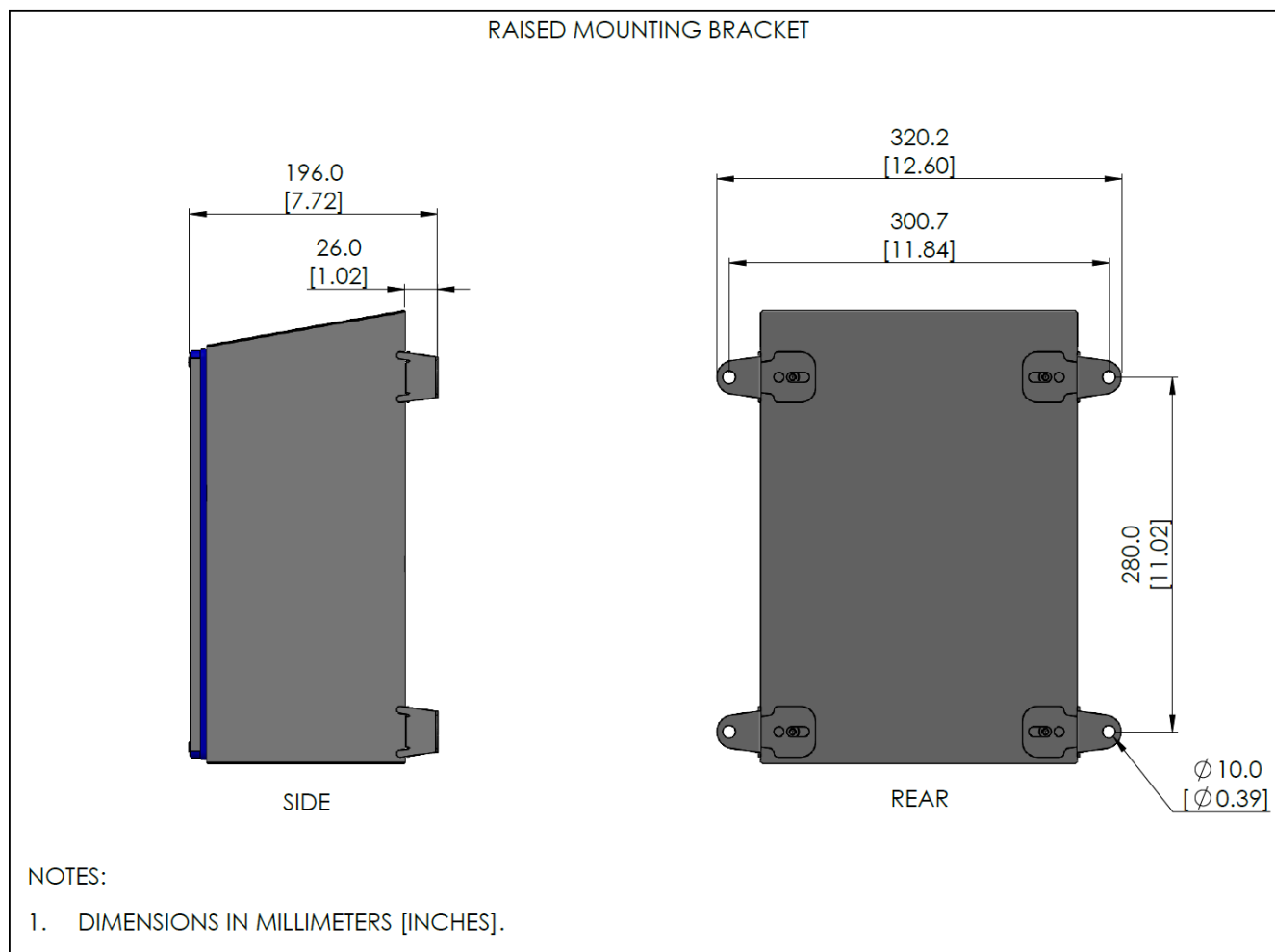
FIGURE 25. AC5000-MNT-03 Raised Mounting Bracket.
