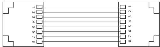
Straight-through Cable
