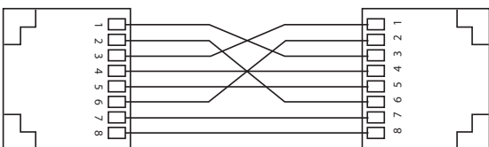
Crossover Cable
