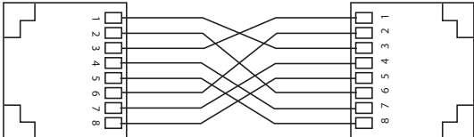
Crossover Cable
