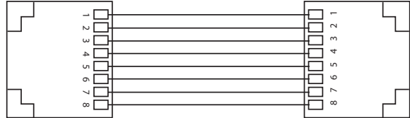
Straight-through Cable
