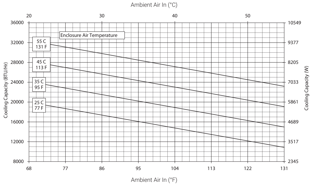
G57-2026-GXXX Capacity Curves at 60 Hz
