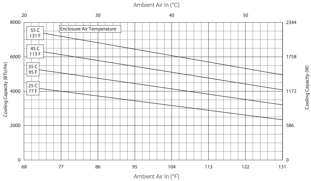
G28-0446-GXXX Capacity Curves at 60 Hz Without Filter
