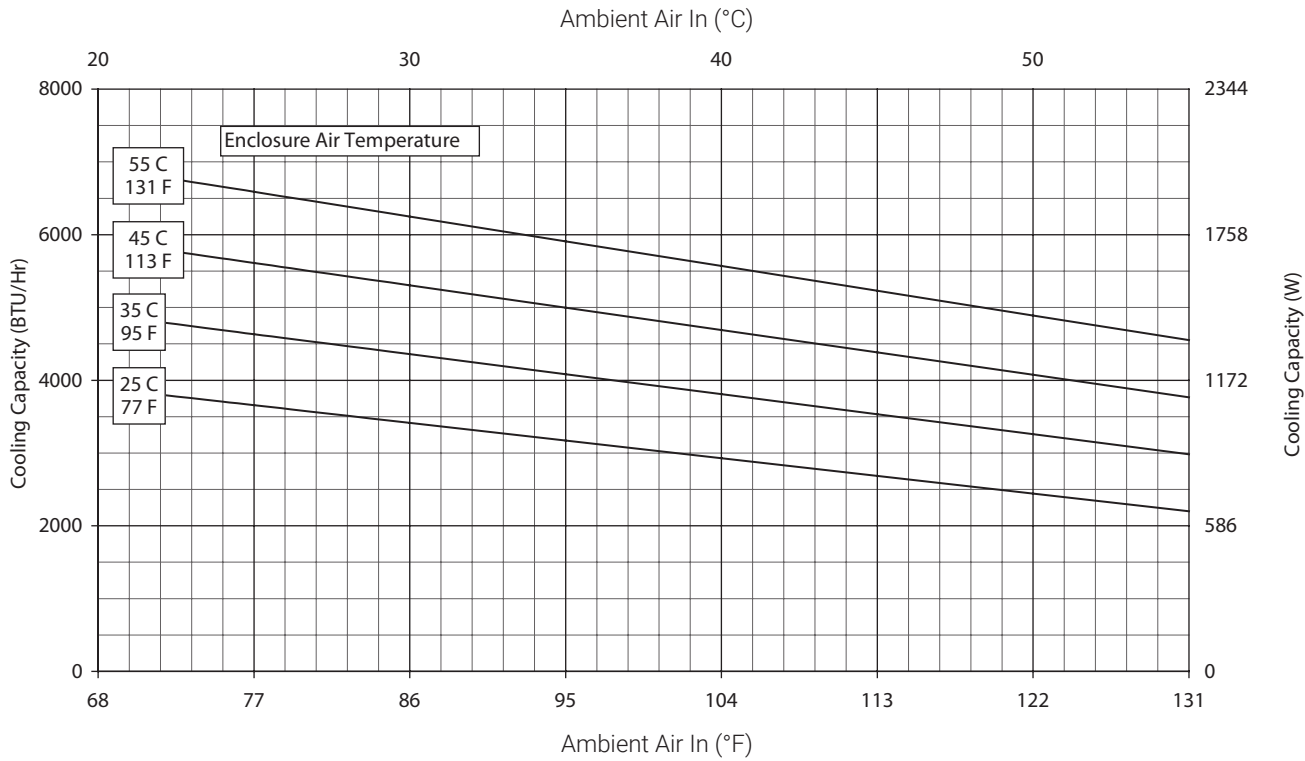
G28-0446-GXXX Capacity Curves at 50 Hz Without Filter
