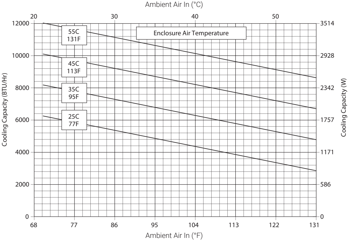
G52-0816-GXXX Capacity Curves at 60 Hz
