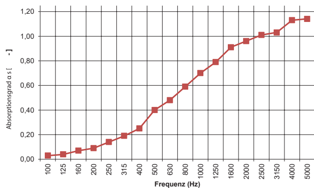
Schallabsorptionskurve Labormessung Recytex 15mm sound absorbtion, labratory test with Recytex 15mm
