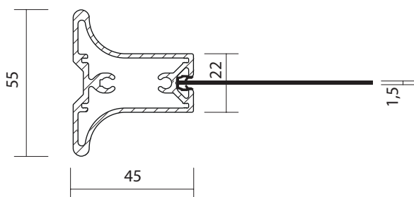
Grundblech in Nut base panels in notch
