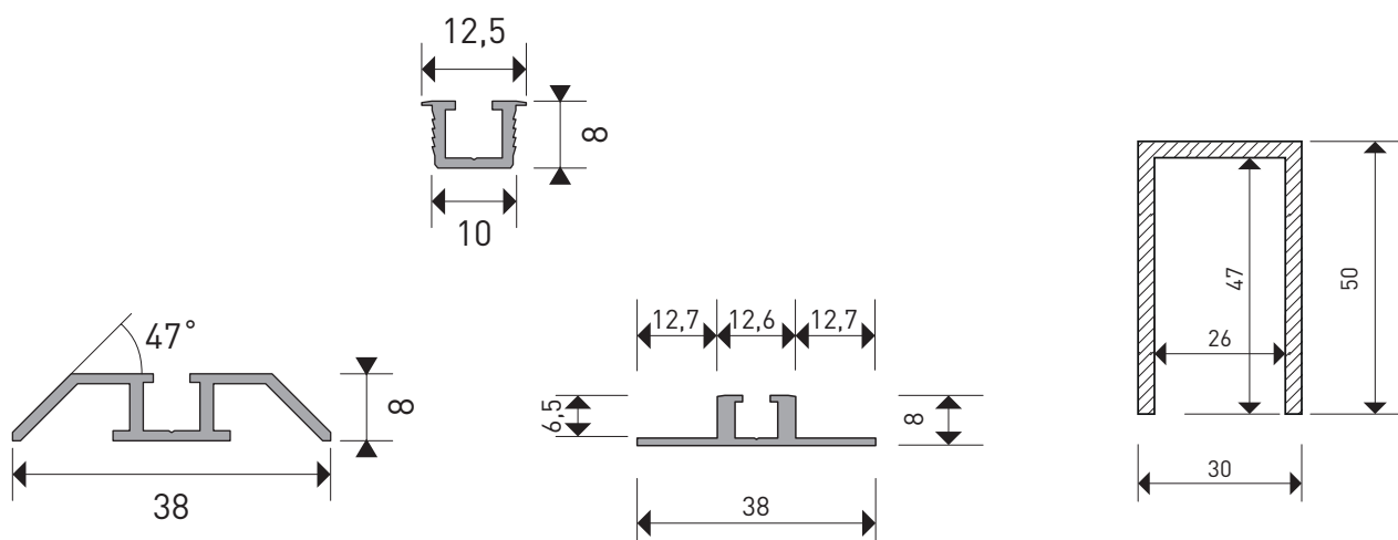
Bodenschiene floor track
