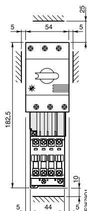
MS325 + BEA16/325AL + AL9...AL16
