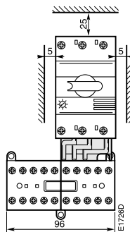
MS325 + BEA7/325 + VB6/VB7
