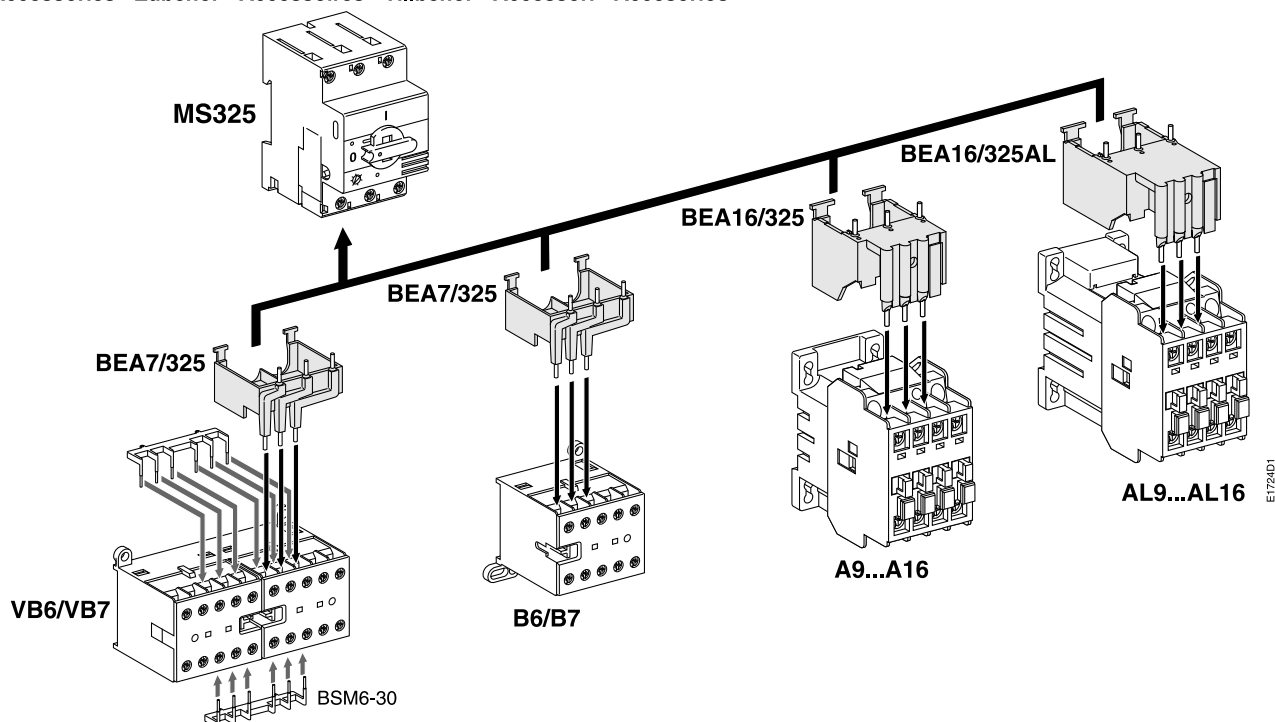
MS325 + BEA16/325 + A9...A16
