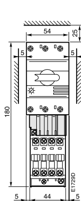
MS325 + BEA16/325 + A9...A16
