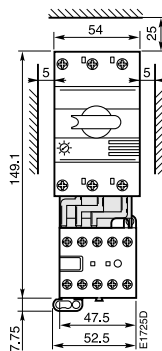
MS325 + BEA7/325 + B6/B7
