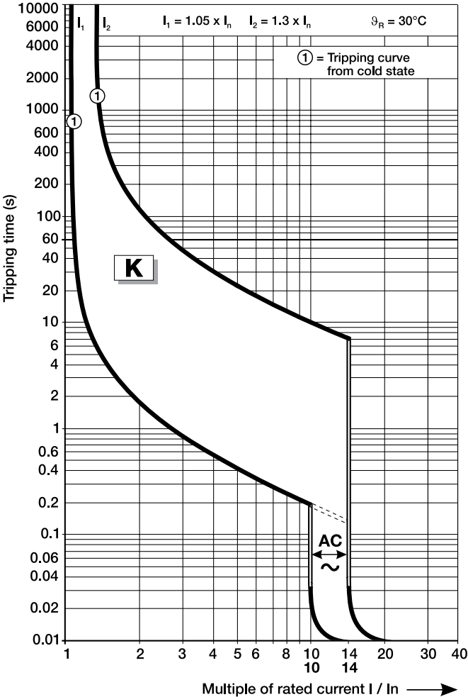
K characteristic
