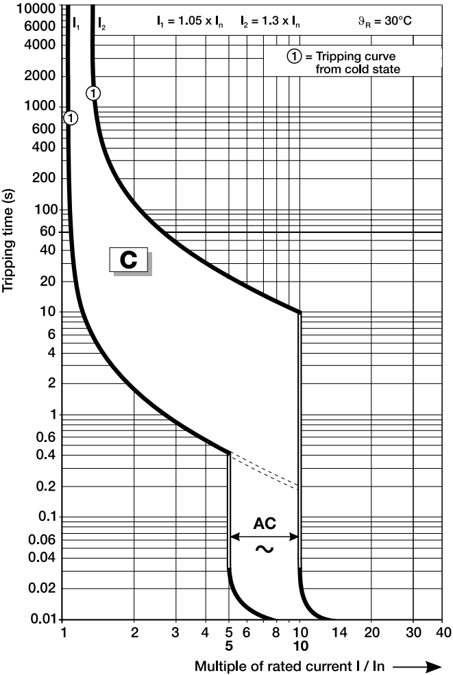
C characteristic
