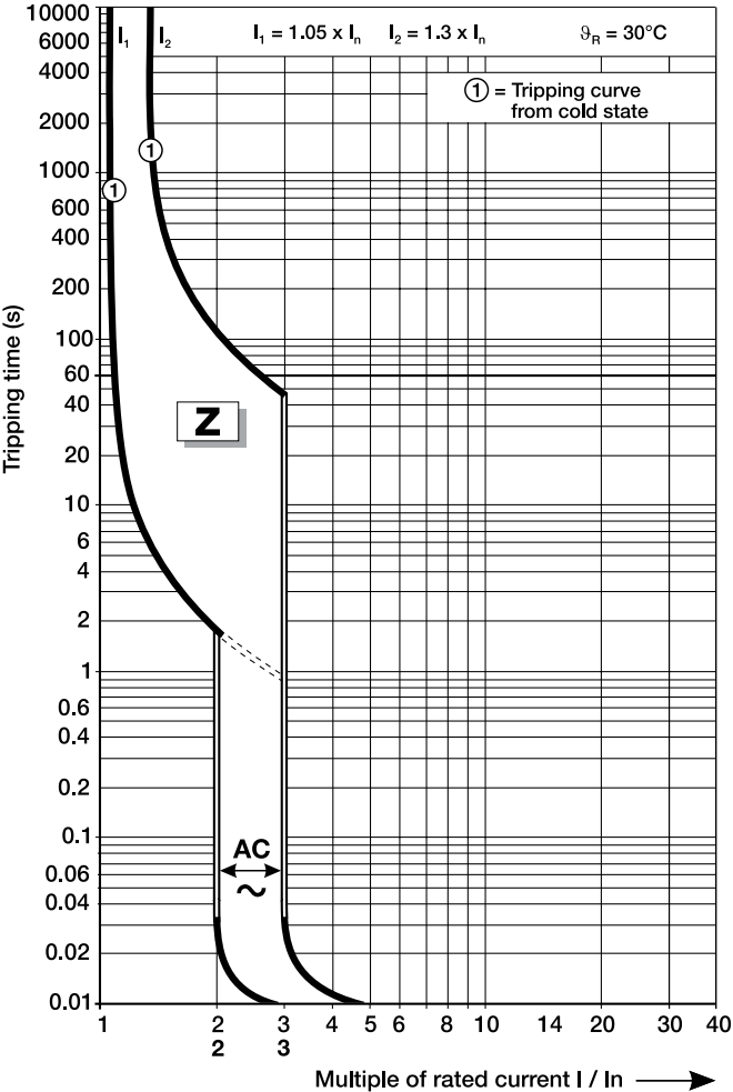
Z characteristic
