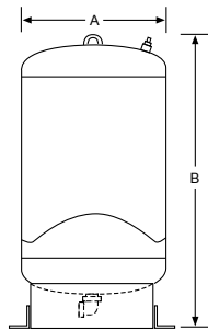
AX-120V through AX-240V Optional restraints shown.
