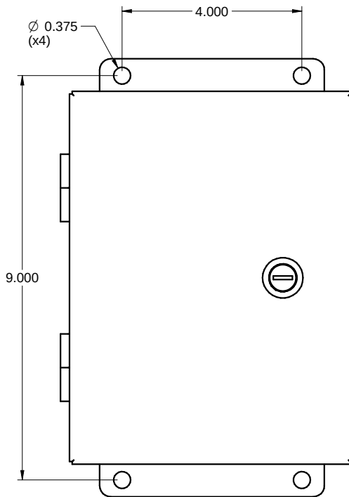
FRONT / FACE
