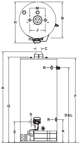
Models ULG250H553N & ULG275H763N
