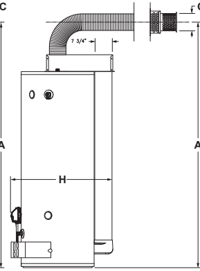
Flexible Vent Kit (Side View)
