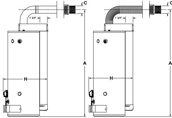
Telescoping Solid Vent Kit (Side View)
