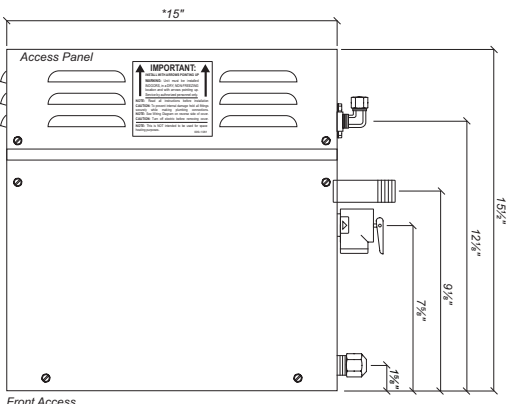
Front Access
