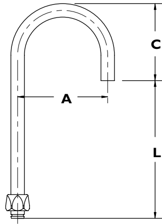
GROUP No. 2 GOOSENECK SMOOTH END (FLOW CONTROL IN BASE OF SPOUT)
