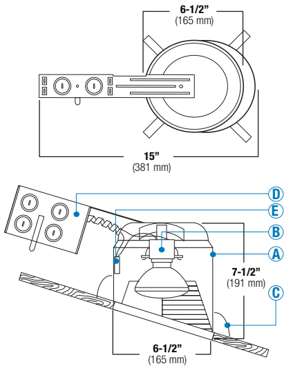
DESIGNED FOR 2" X 8" JOIST CONSTRUCTION
