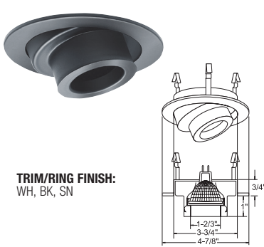
B1427CL-WH THE ILLUMINATOR
