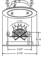
B1466CL-WH ADJUSTABLE ANGLE-CUT SLOT APERTURE
