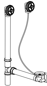
Fig. C Tubular Remote Control Rough-In Unit
