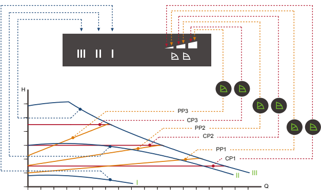
Fig. 1 Pump setting in relation to pump performance
