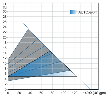
Proportional pressure
