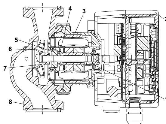
Fig. 50 Wire-to-wire-connected version
