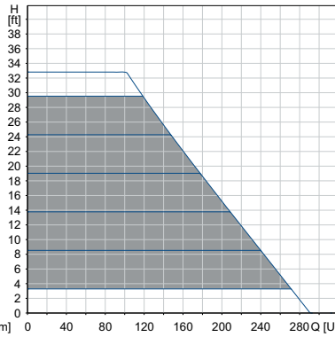
Constant pressure
