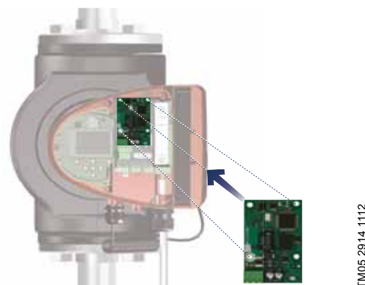
Fig. 60 Location of CIM module
