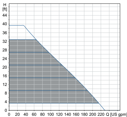
Constant pressure
