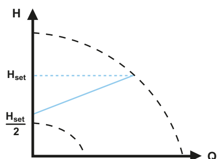
Fig. 18 Proportional-pressure control
