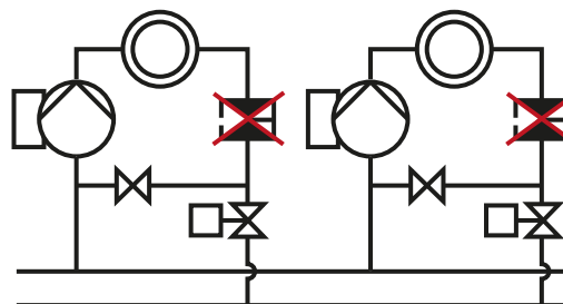
Fig. 17 Reduced need for a pump throttling valve
