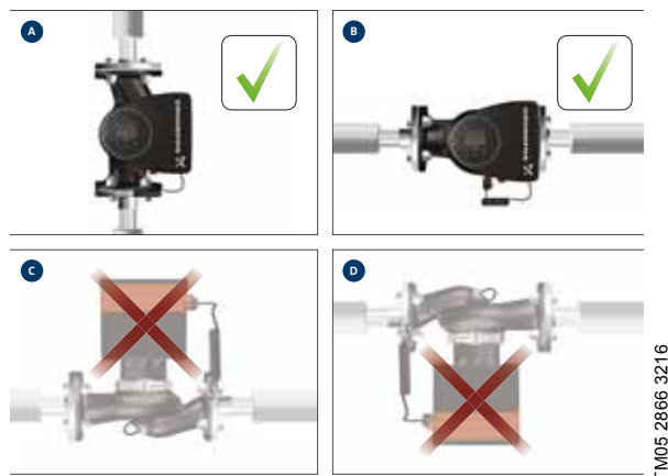
Fig. 52 Installation positions
