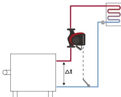
Fig. 24 Differential temperature
