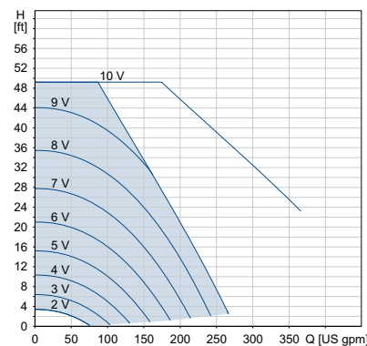
0-10 volt*
