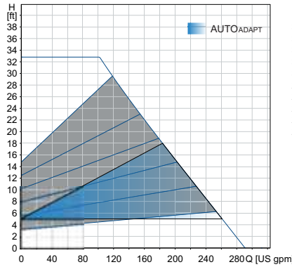
Proportional pressure
