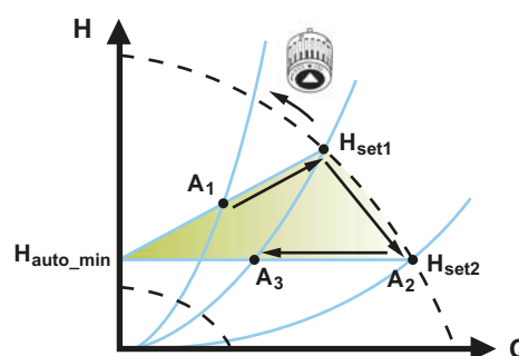
Fig. 15 AUTO_{ADAPT} control
