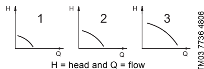
Fig. 13 Pump performance at speed settings
