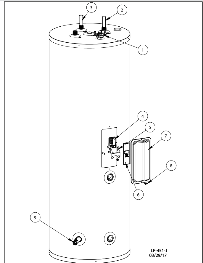
Figure 10 - Replacement Parts
