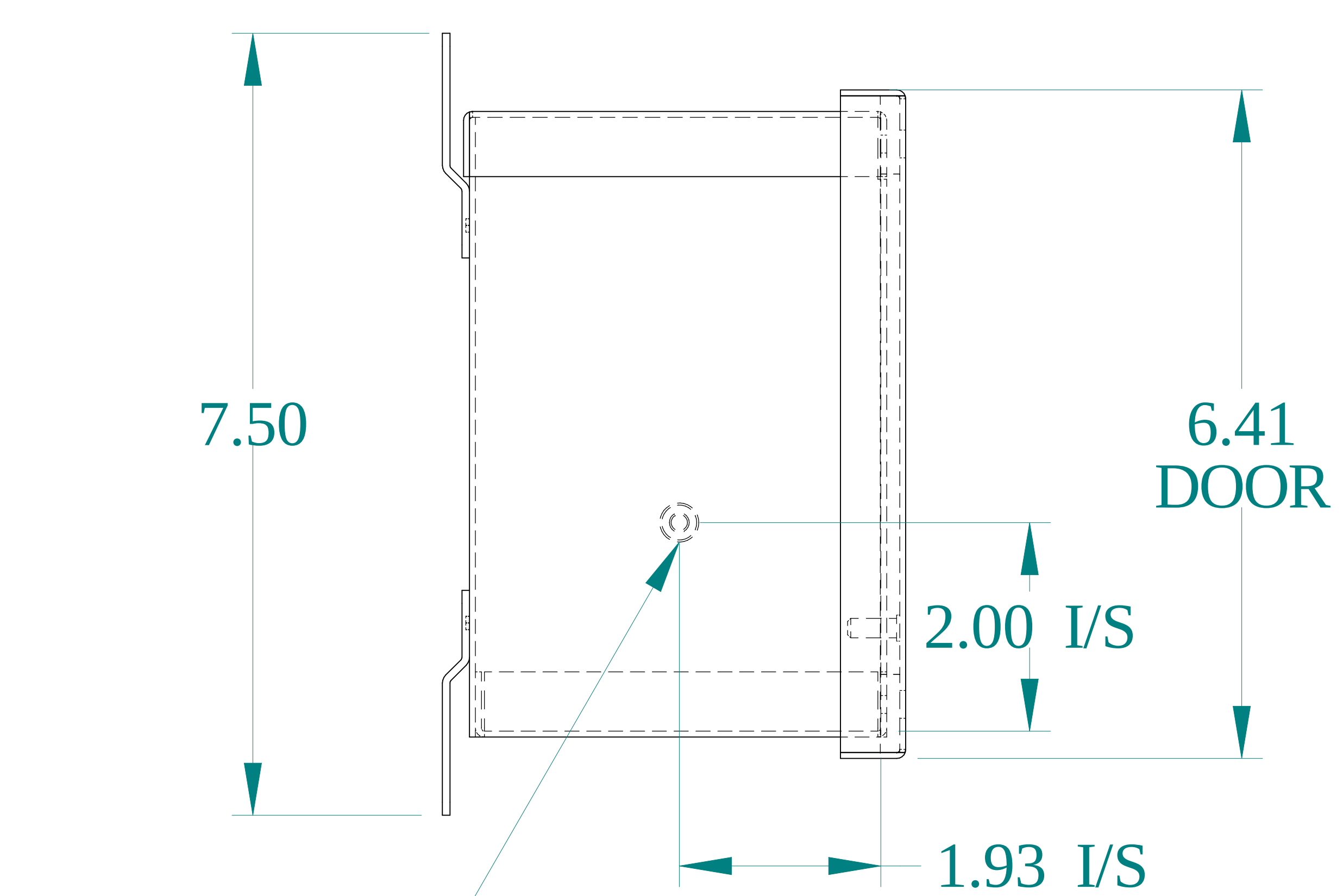
GROUND STUD BODY SIDE VIEW
