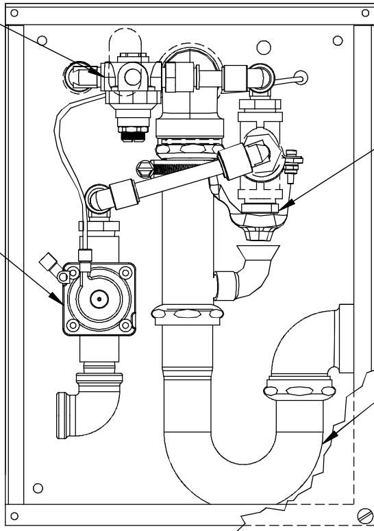
5867 REGULATOR ASSEMBLY
