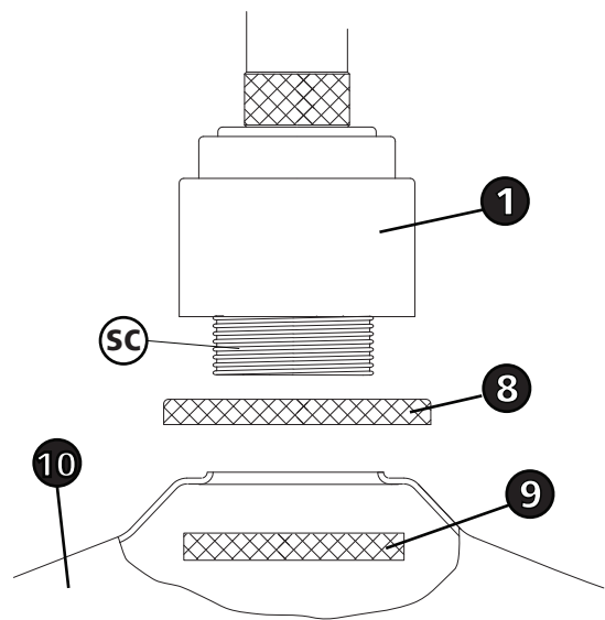
DRAWING 1 - SHADE INSTALLATION
