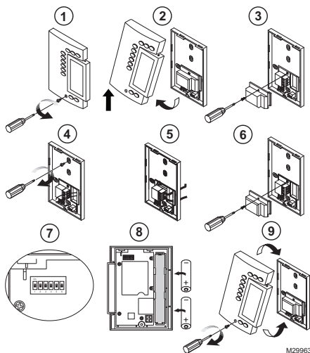
Fig. 1. Installation steps.
