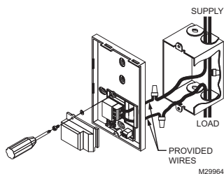
Fig. 2. Routing wires to thermostat.
