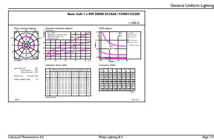
LEDbulb, Bulb A19 8W-60W 5000K 800lm
