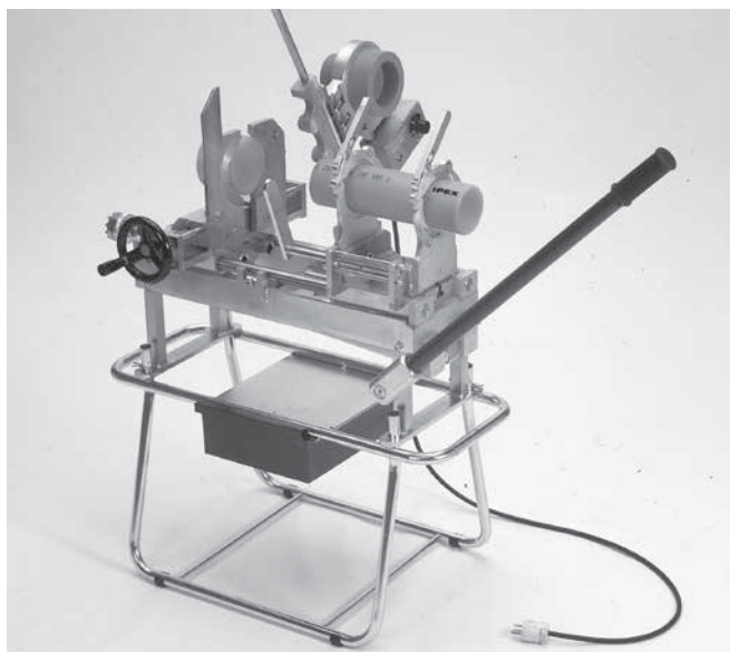
Socket Fusion Tool Kit c/w Full Set of Heater Bushings 110V, 50Hz
