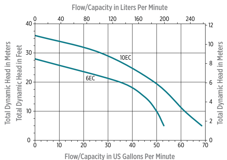
6EC - SPBS-10HF-6, 1/3 hp Primary Pump
