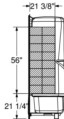
OPTIONAL REINFORCEMENT (Left shown, Right symmetrical)
