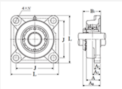
Four Bolt Square Flanged Unit, Cast Housing, Adapter, UKF Type - Dimensions
